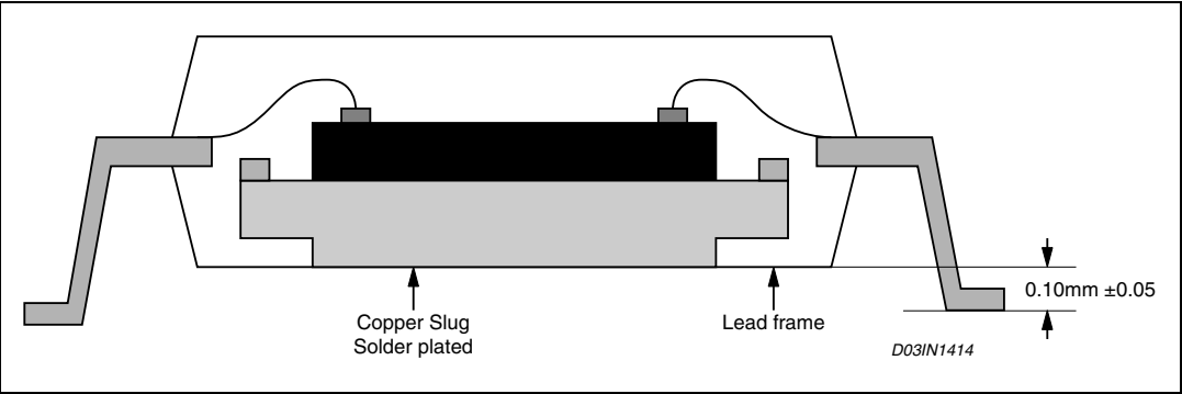
Figure 26. ST7538Q slug drawing
