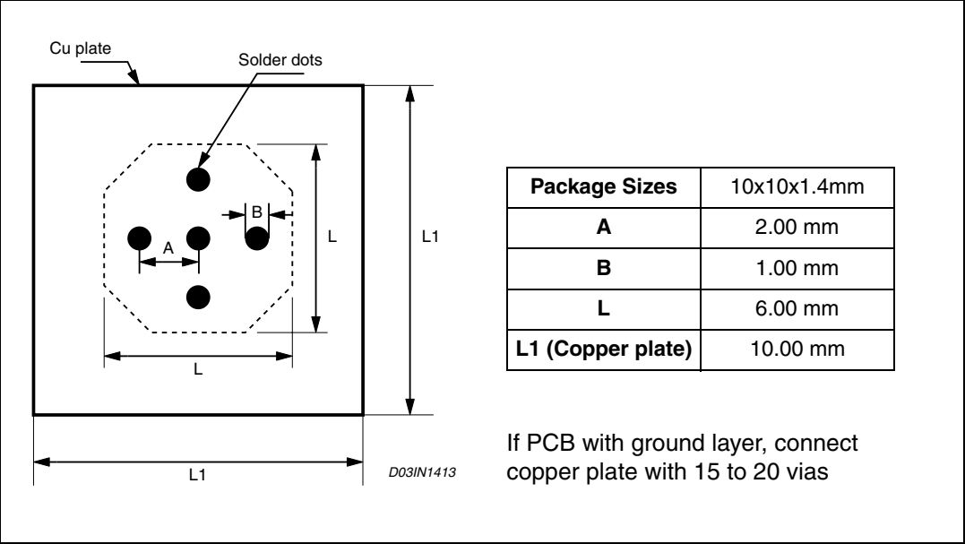
Figure 27. Soldering information
