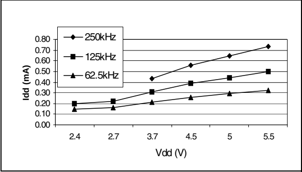
Figure 57. Typical I_{DD} in SLOW vs. f_{CPU}
