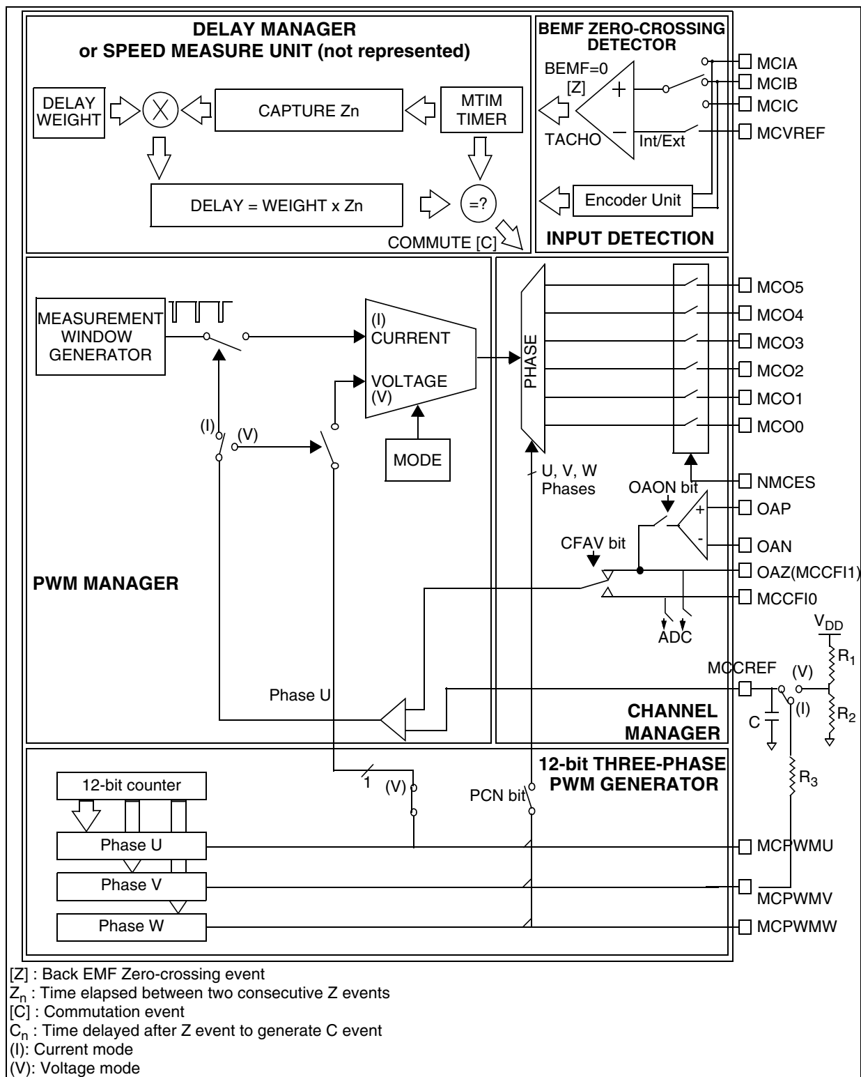
Figure 77. Simplified MTC Block Diagram
