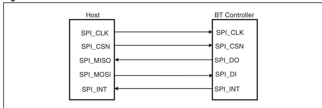
Figure 16. SPI interface
