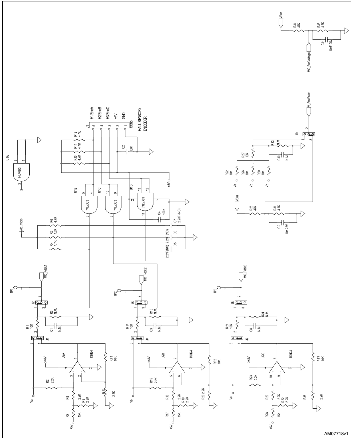
Figure 16. Bemf_hall_encoder schematic
