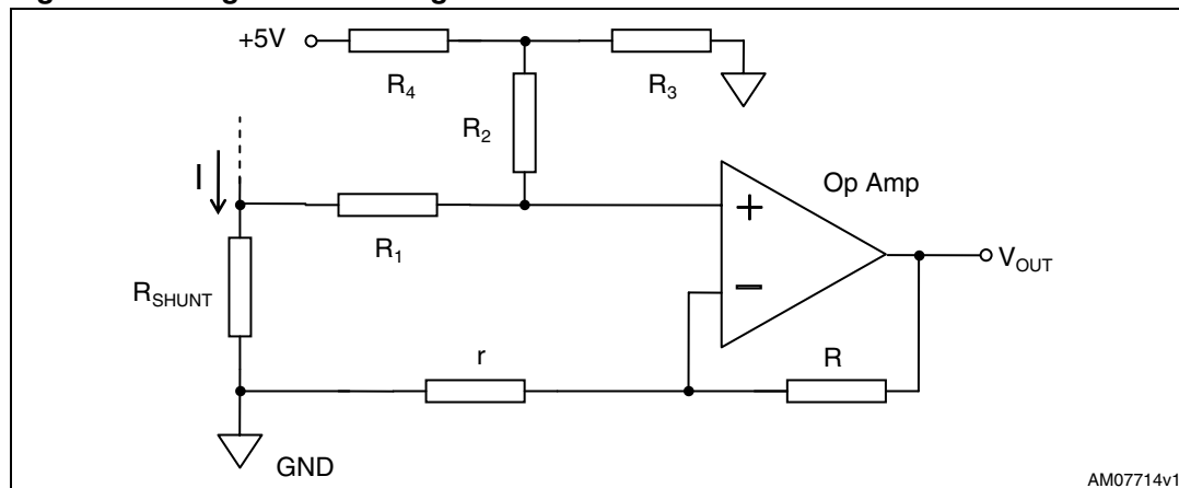
Figure 12. Single-shunt configuration
