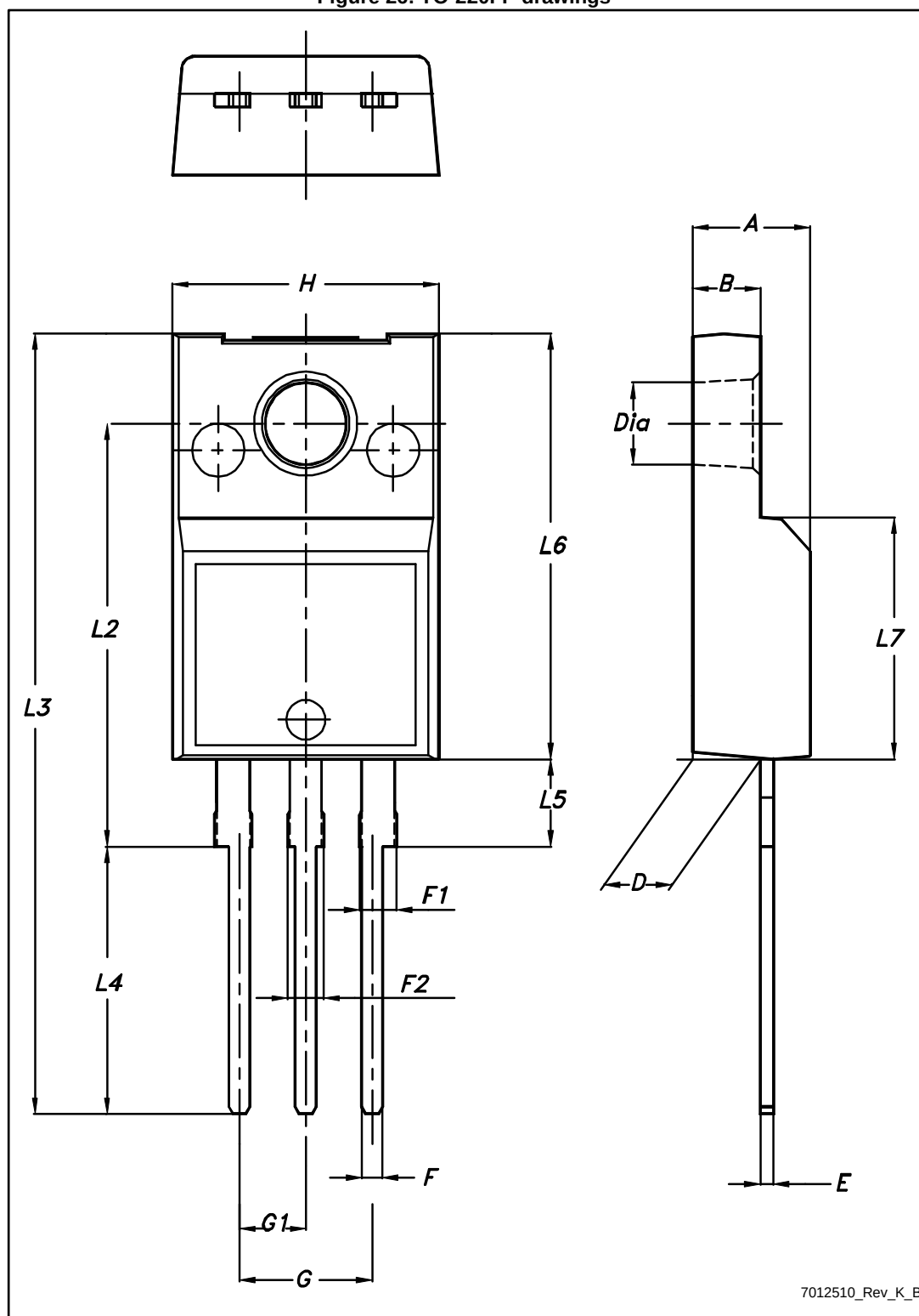
Figure 26: TO-220FP drawings
