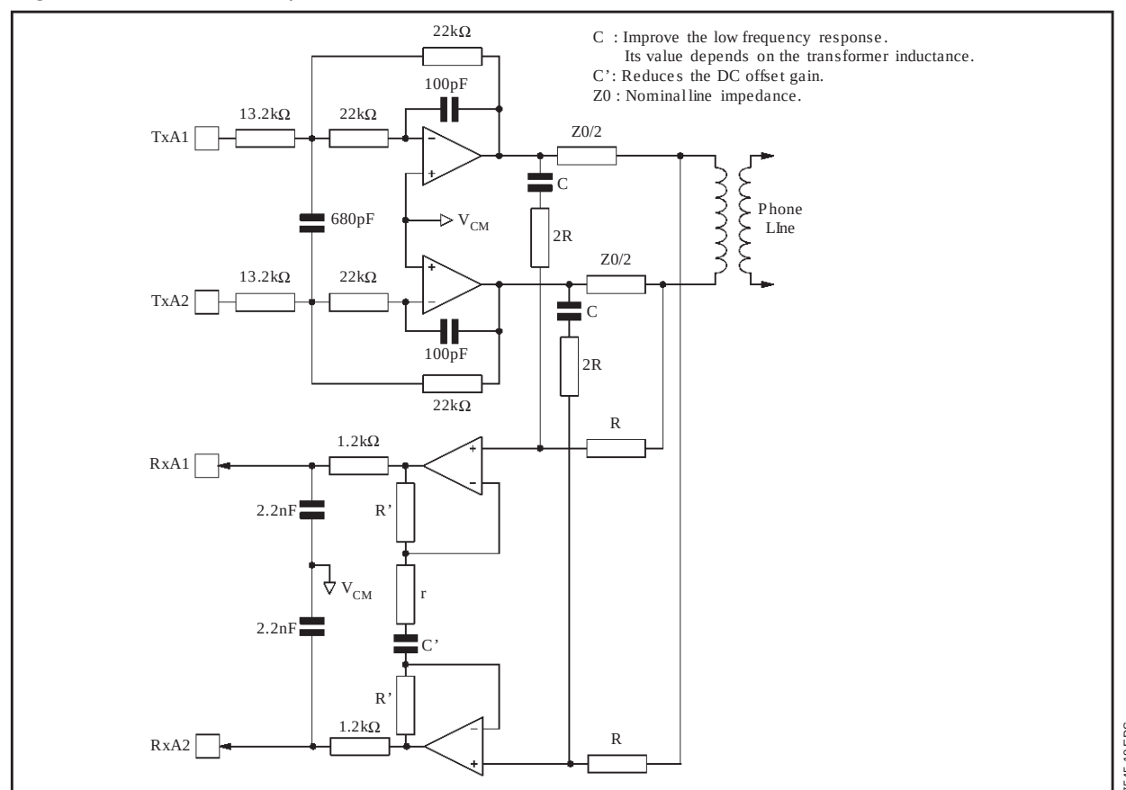
Figure 16 : Differential Duplexer
