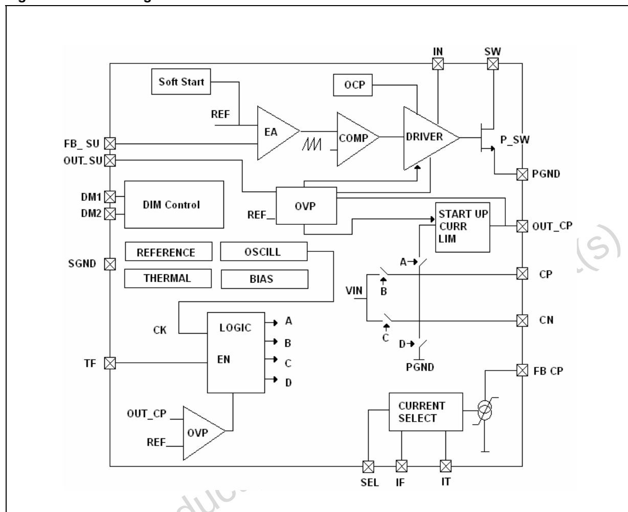
Figure 1. Block diagram
