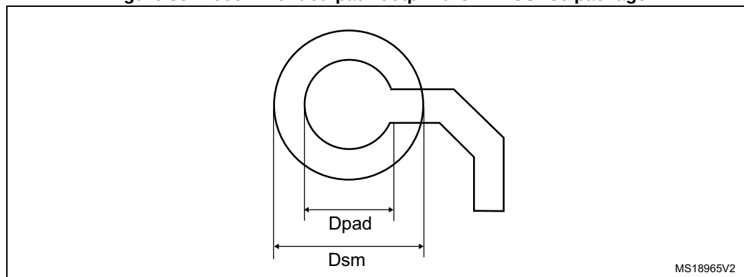
Figure 33. Recommended pad footprint for WLCSP36 package
