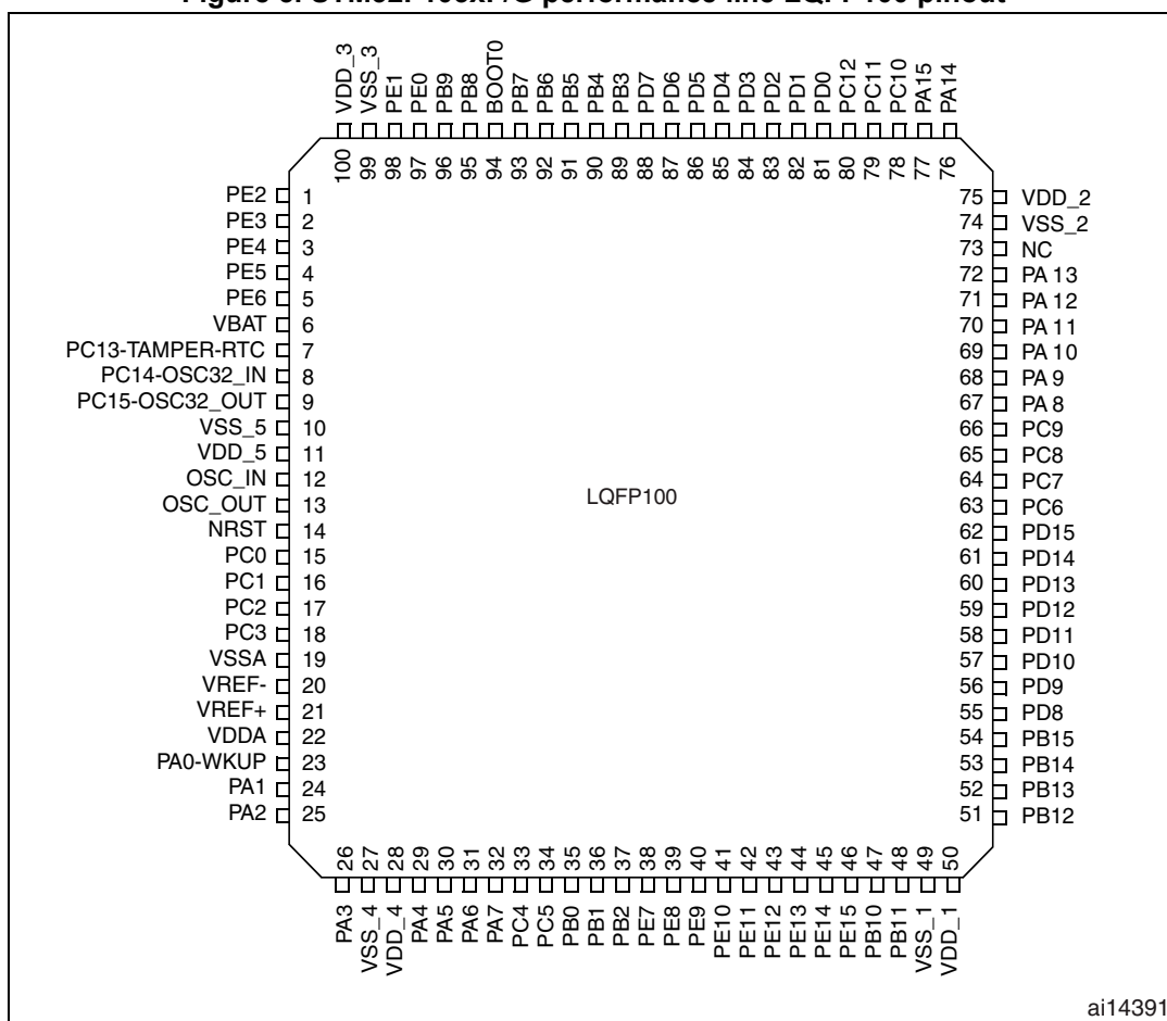
Figure 5. STM32F103xF/G performance line LQFP100 pinout
