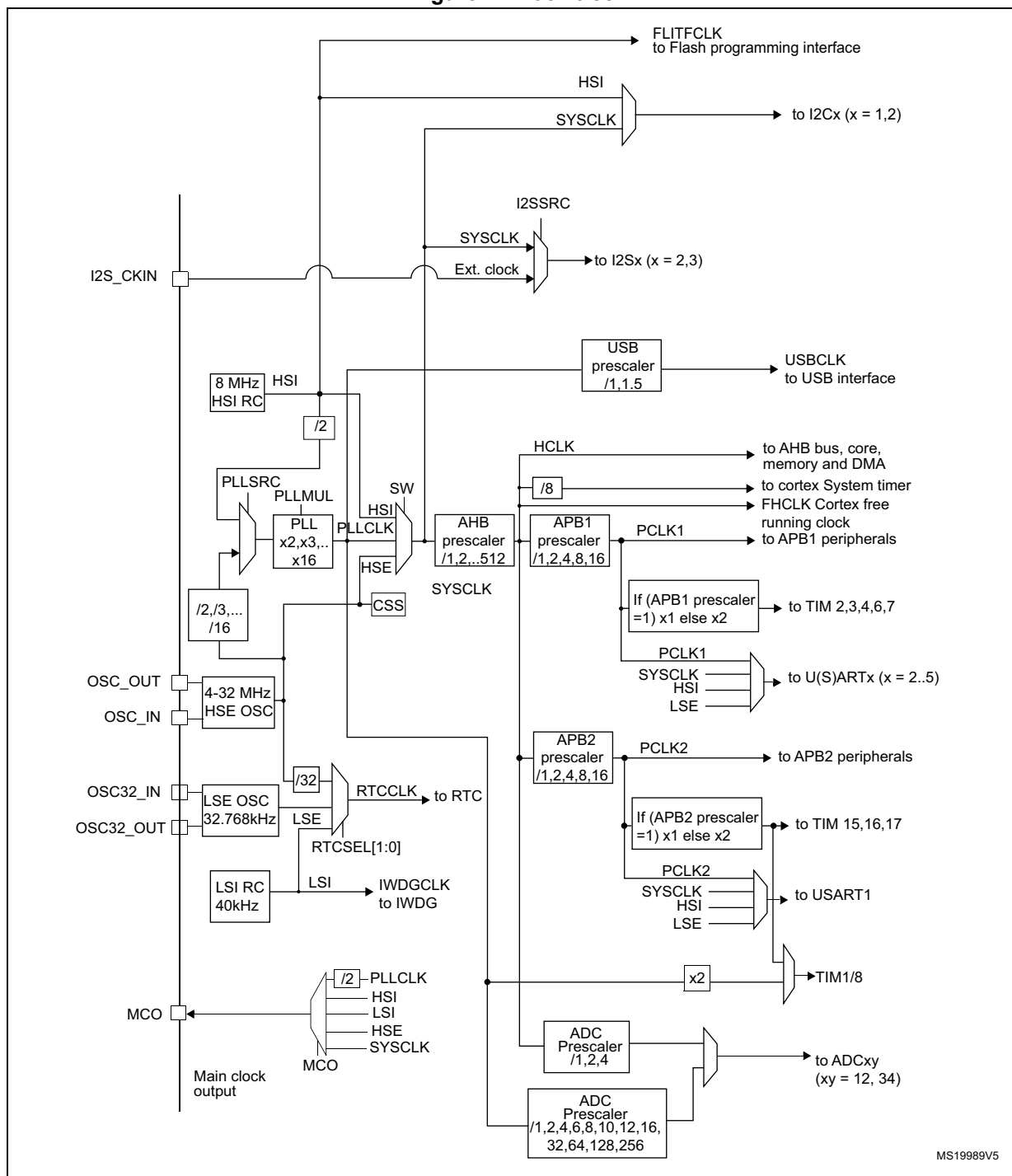
Figure 2. Clock tree
