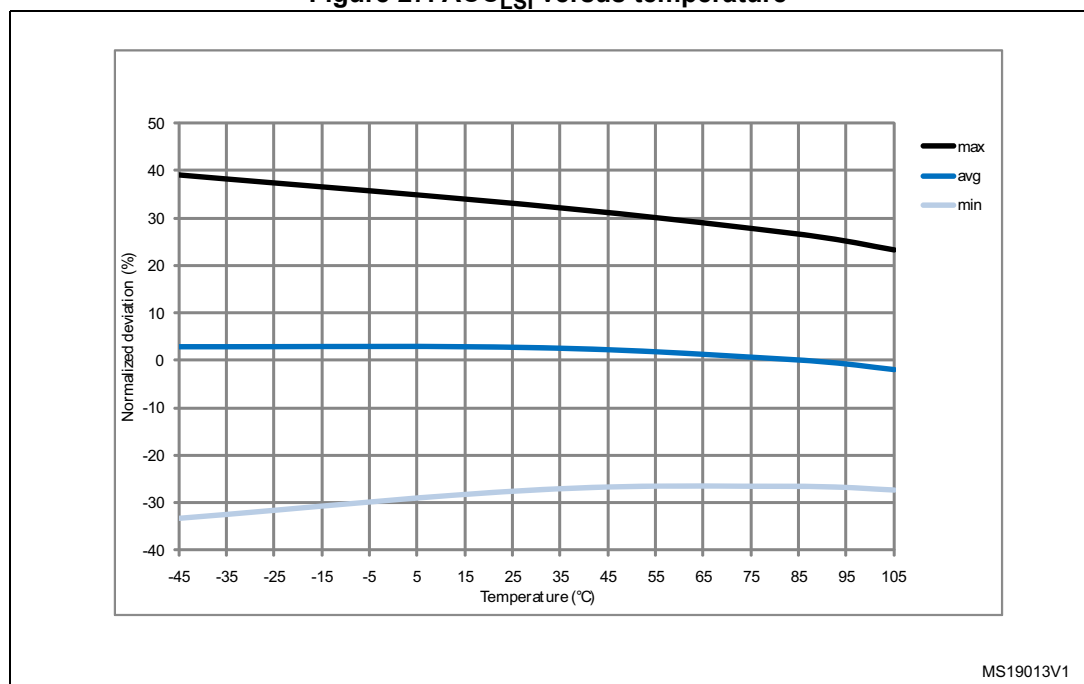
Figure 27. \text{ACC}_{\text{LSI}} versus temperature
