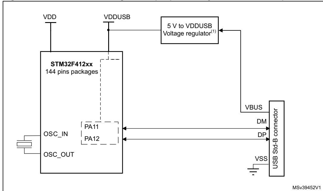
Figure 75. USB controller configured as peripheral-only and used in Full speed mode
