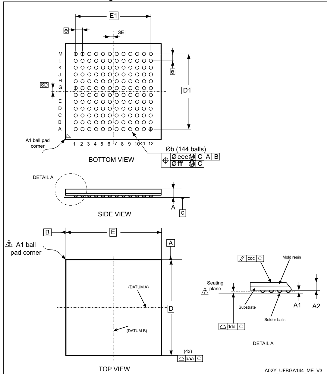
Figure 73. UFBGA144 - Outline (13)
