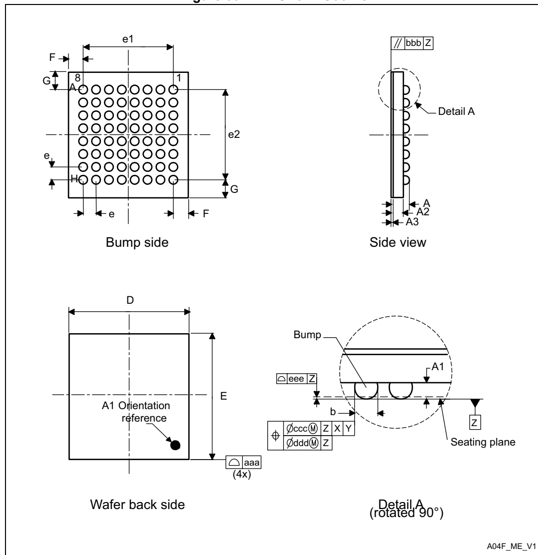
Figure 60. WLCSP64 - Outline
