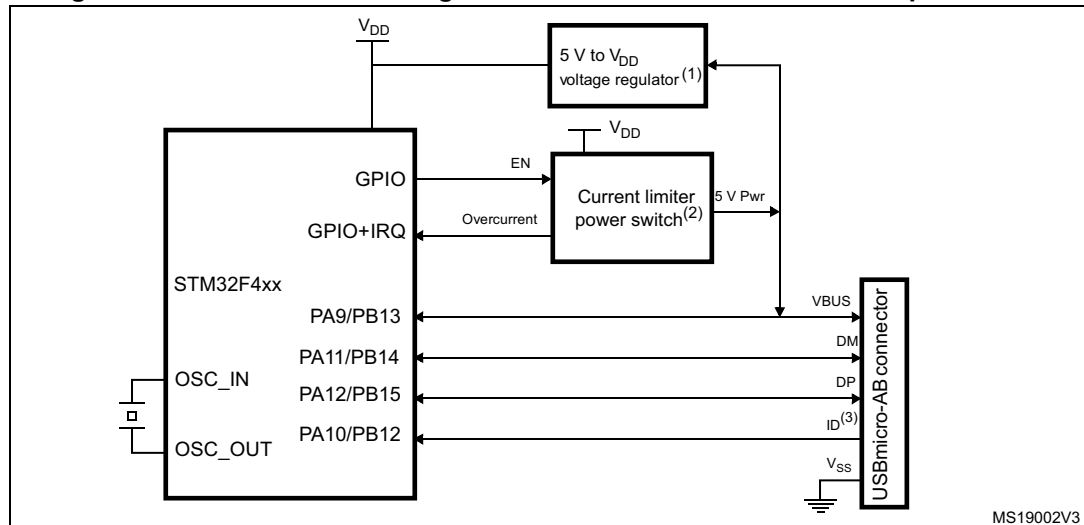
Figure 97. USB controller configured in dual mode and used in full speed mode
