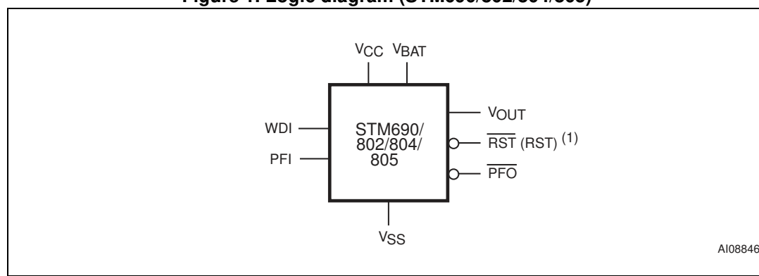
Figure 1. Logic diagram (STM690/802/804/805)
