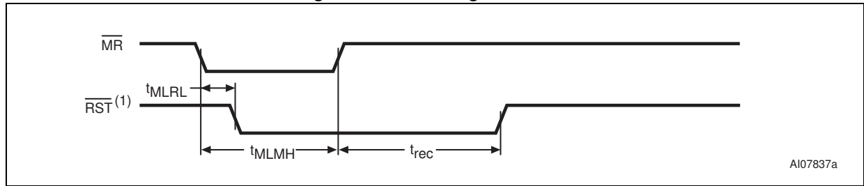
Figure 36. \overline{\text{MR}} timing waveform
