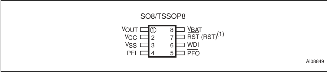
Figure 4. STM690/802/804/805 connections
