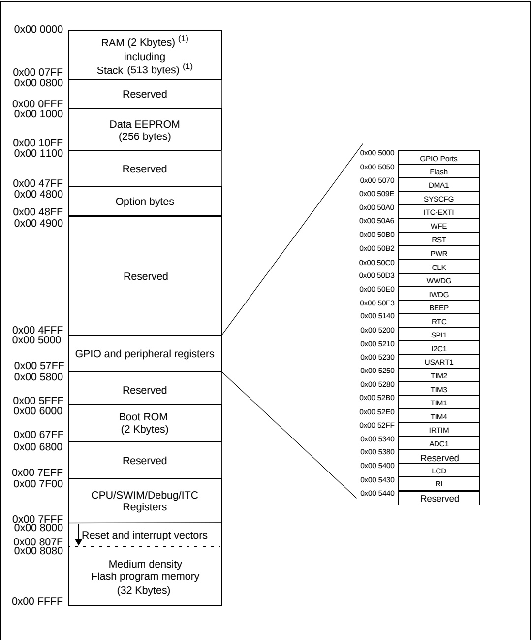
Figure 4. Memory map
