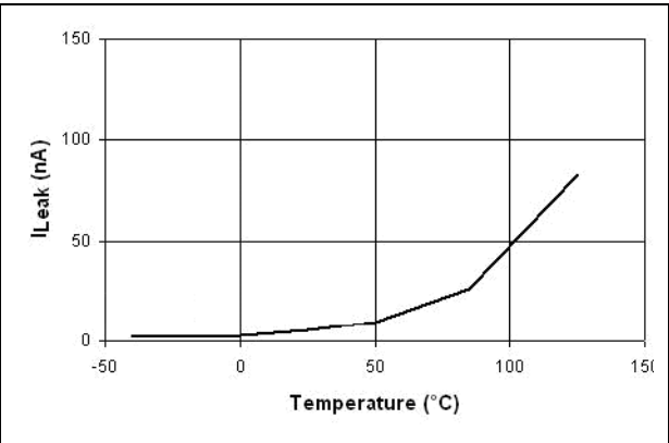
Figure 49. Switch leakage vs. temperature (STMP2161/2171)
