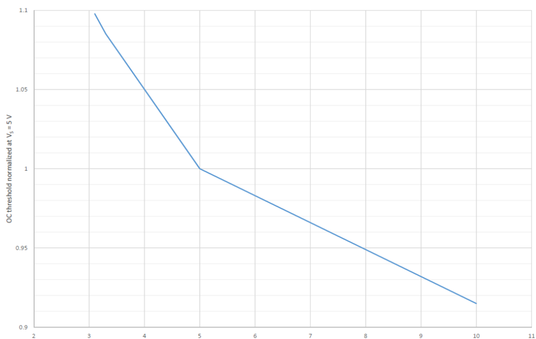
Figure 15. Overcurrent threshold versus supply voltage
