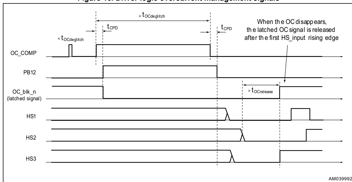
Figure 16. Driver logic overcurrent management signals
