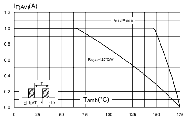
Figure 3. Average forward current versus ambient temperature (δ = 0.5) (SMA)
