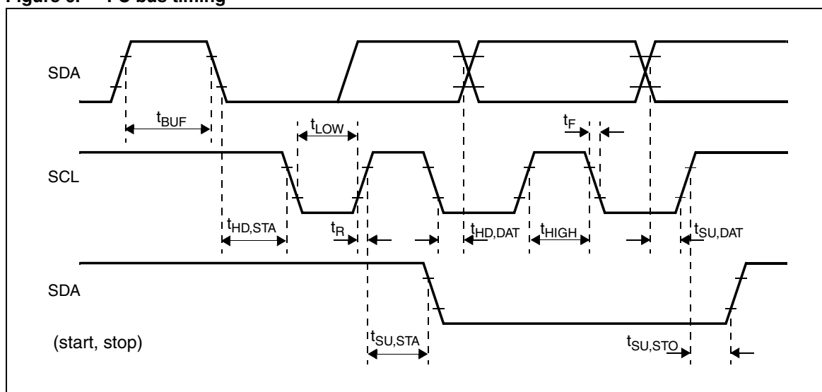
Figure 6. I 2 C bus timing
