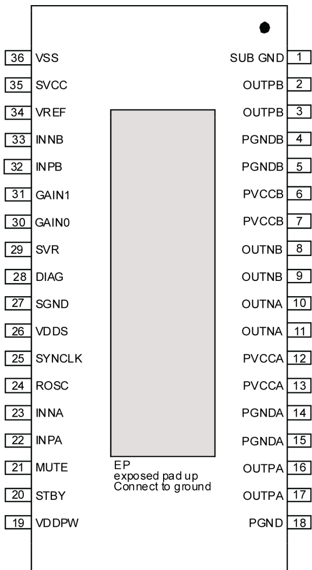
Figure 3. Pin connections (top view)
