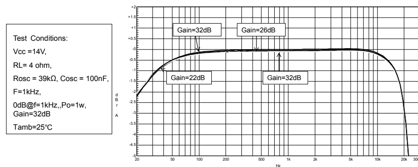
Figure 14. Closed-loop gain vs. frequency
