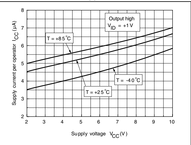
Figure 10. Supply current ( I_{CC} ) vs. supply voltage ( V_{CC} ) ( V_{ID} = +1\text{ V} )
