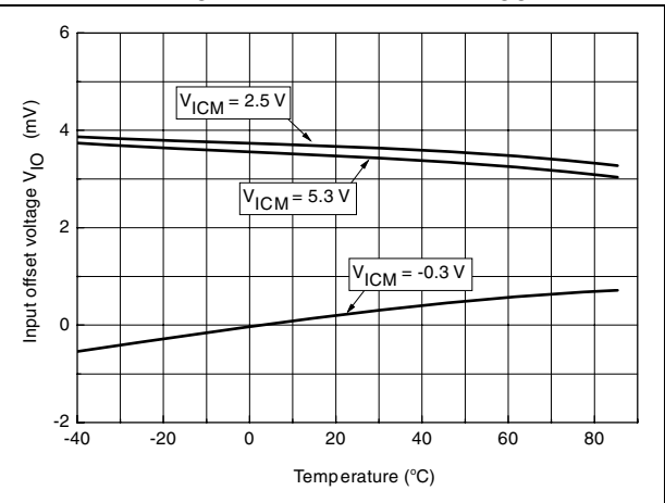
Figure 8. V_{IO} vs. temperature at V_{CC} = 5\text{ V}
