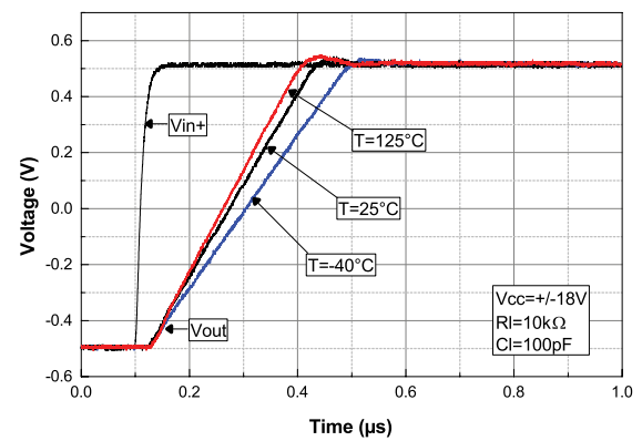
Figure 20. Positive slew rate at V_{CC} = 36\text{ V}
