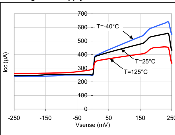
Figure 5. Supply current vs. Vsense
