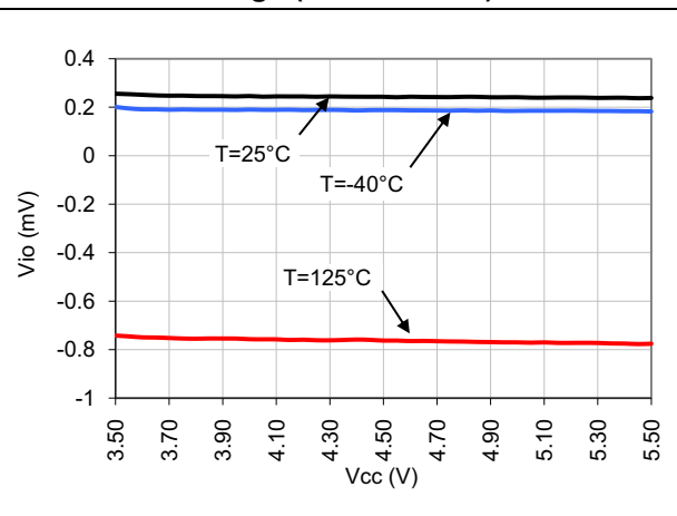
Figure 15. Input offset voltage versus supply voltage ( V_{\text{cm}} = V_{\text{CC}}/2 )
