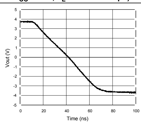
Figure 37. Large signal measurement - negative slew rate (gain = 2, V_{CC} = \pm 5\text{ V} , Z_L = 150\ \Omega // 5.6\text{ pF} )
