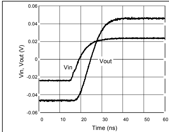
Figure 23. Small signal measurement - rise time (gain = 2, V_{CC} = \pm 2.5 V, Z_L = 150 \Omega )
