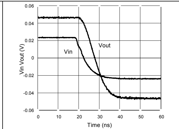
Figure 24. Small signal measurement - fall time (gain = 2, V_{CC} = \pm 2.5 V, Z_L = 150 \Omega )
