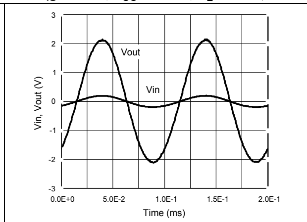
Figure 28. Maximum output swing (gain = 11, V_{CC} = \pm 2.5 V, R_L = 150 \Omega )
