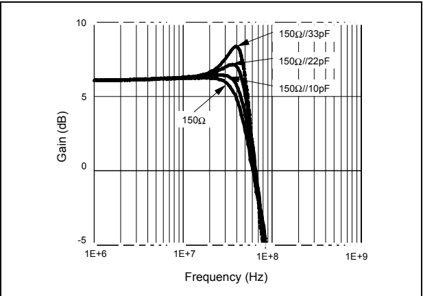
Figure 3. Overshoot function of output capacitance (gain = +2, V_{CC} = \pm 1.5\text{ V} , T_{amb} = 25\text{ }^\circ\text{C} )
