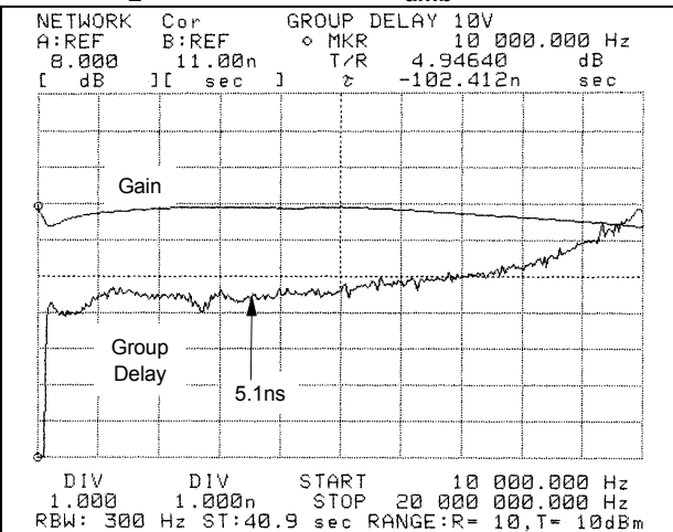
Figure 45. Group delay (gain = 2, V_{CC} = \pm 5 V Z_L = 150 \Omega // 27 pF, T_{amb} = 25 °C)
