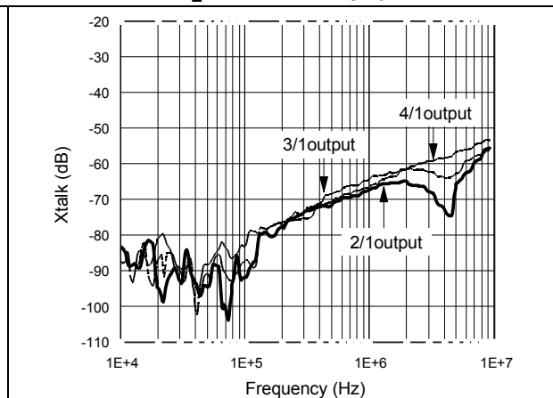
Figure 26. Channel separation (Xtalk) vs. frequency (gain = +11, V_{CC} = \pm 2.5 V, Z_L = 150 \Omega // 27 pF)
