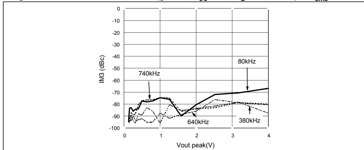
Figure 46. Third order intermodulation (gain = 2, V_{CC} = \pm 5 V, Z_L = 150 \Omega // 27 pF, T_{amb} = 25 °C
