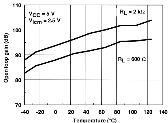
Figure 6. Open loop gain vs. temperature at V_{\text{CC}} = 5\text{ V}
