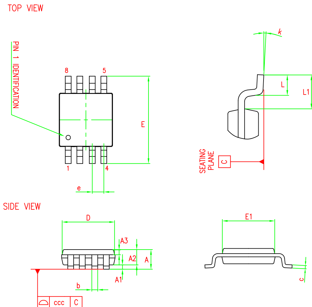
Figure 21. MiniSO8 package outline
