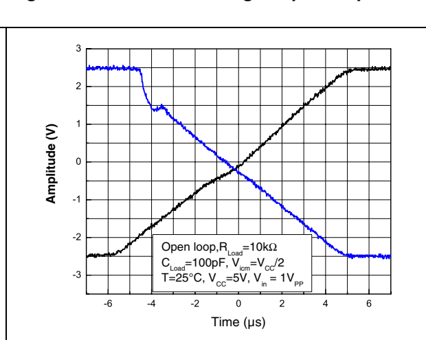
Figure 11. Slew rate timing in open loop
