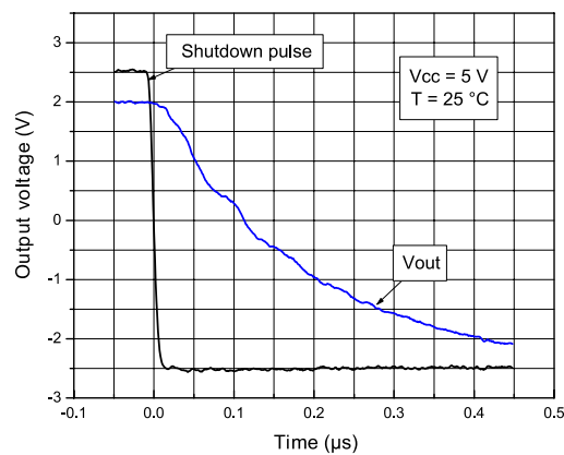
Figure 18: Turn-off time, V_{\text{CC}} = 5 V, Vout pulled down, T = 25 °C
