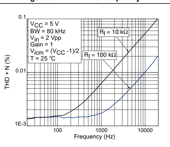
Figure 19. THD+N vs. frequency
