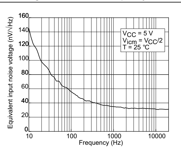
Figure 17. Noise vs. frequency
