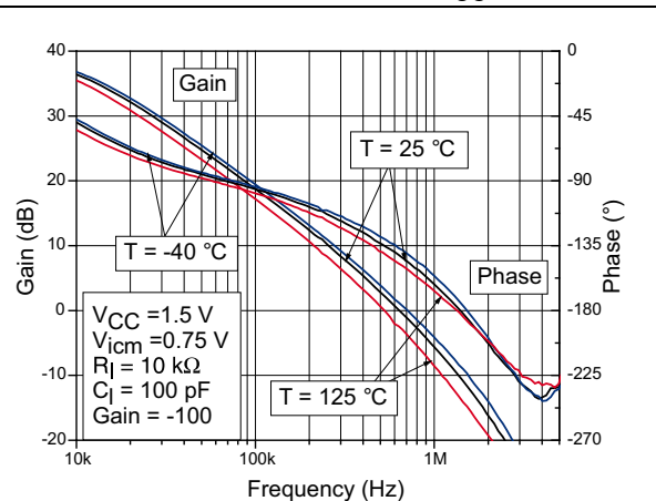
Figure 11. Bode diagram at V_{CC} = 1.5\text{ V}
