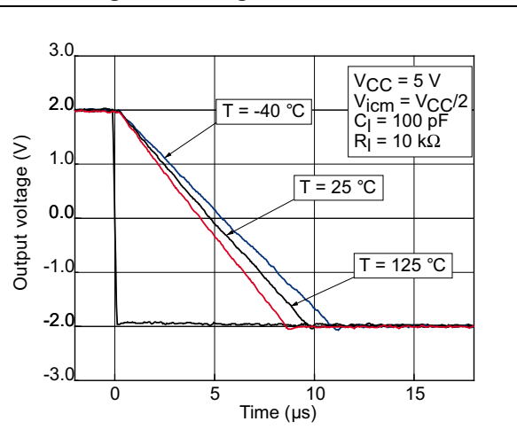
Figure 15. Negative slew rate
