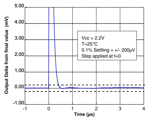
Figure 41. Settling time positive step (-0.8 V to 0 V)
