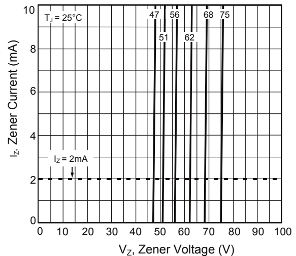
Figure 4. Zener Breakdown Characteristics ( V_Z 47V-75V)
