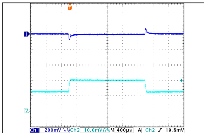
Figure 5: Output voltage response to step-change in load current (50% -75% -50% of I out (max); dI/dt = 0.1 A/μs). Load cap: 100 μF electrolytic capacitor. Ch 1: V out (200 mV/div), Ch 2: I out (10 A/div).
