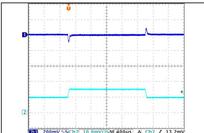
Figure 5: Output voltage response to step-change in load current (50 %-75 % -50 % of I out (max); dI/dt = 0.2 A/μs). Load cap: 100 μF electrolytic capacitor. Ch 1: V out (200mV/div), Ch 2: I out (10 A/div).
