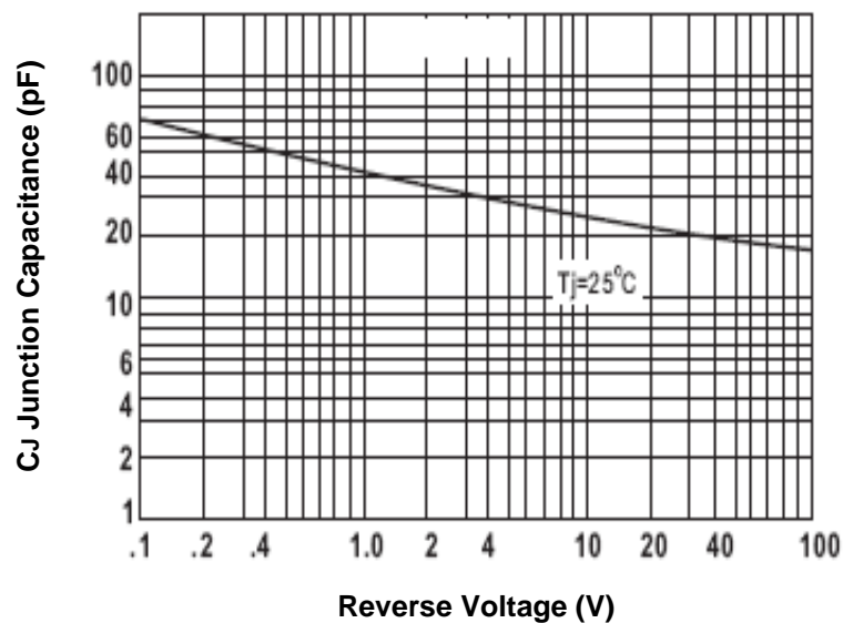
Fig.5-Typical Junction Capacitance
