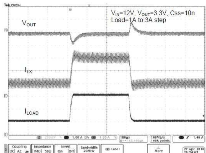
Figure 6. Load Transient
