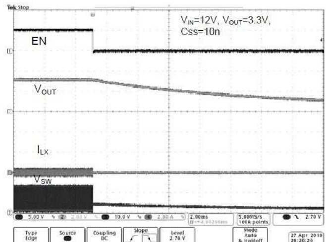
Figure 4. Shutdown Waveform at I_{OUT}=0\text{A}
