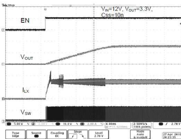
Figure 3. Start-Up Waveform at I_{OUT}=3\text{A}
