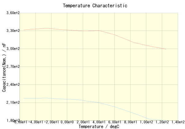
C3216X7R2A334K130AA(DC Bias = 0V) C3216X7R2A334K130AA(DC Bias = 50V)
