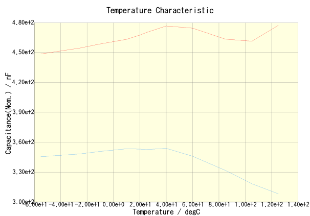
C3225X7R2A474K200AA(DC Bias = 0V) C3225X7R2A474K200AA(DC Bias = 50V)
