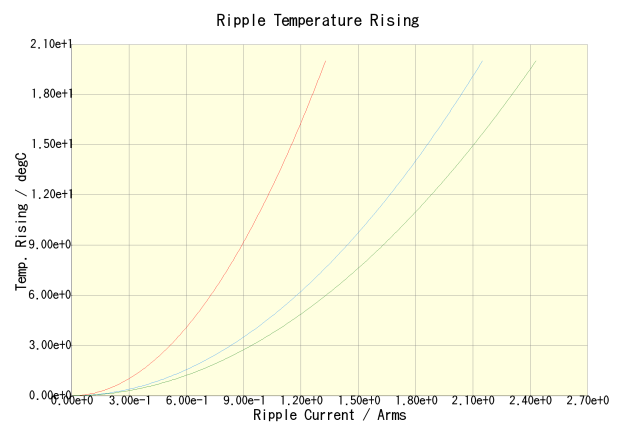
C3225X7R2A474K200AA(100kHz) C3225X7R2A474K200AA(500kHz) C3225X7R2A474K200AA(1MHz)
