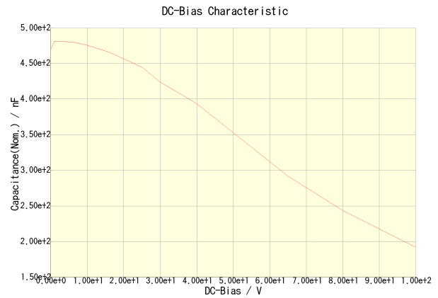
C3225X7R2A474K200AA
