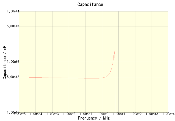
C3225X7R2A474K200AA
