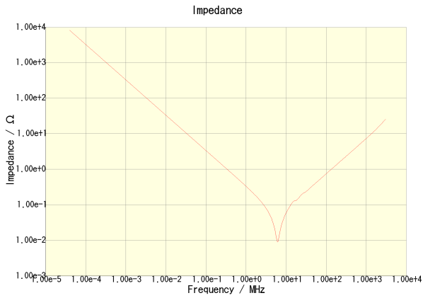
C3225X7R2A474K200AA
