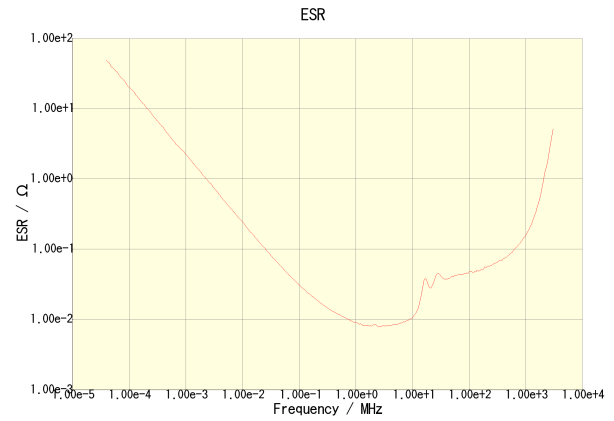
C3225X7R2A474K200AA
