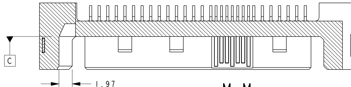
SECTION M - M SCALE 3:1
