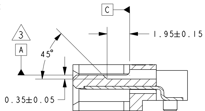
SECTION G - G SCALE 5:1
