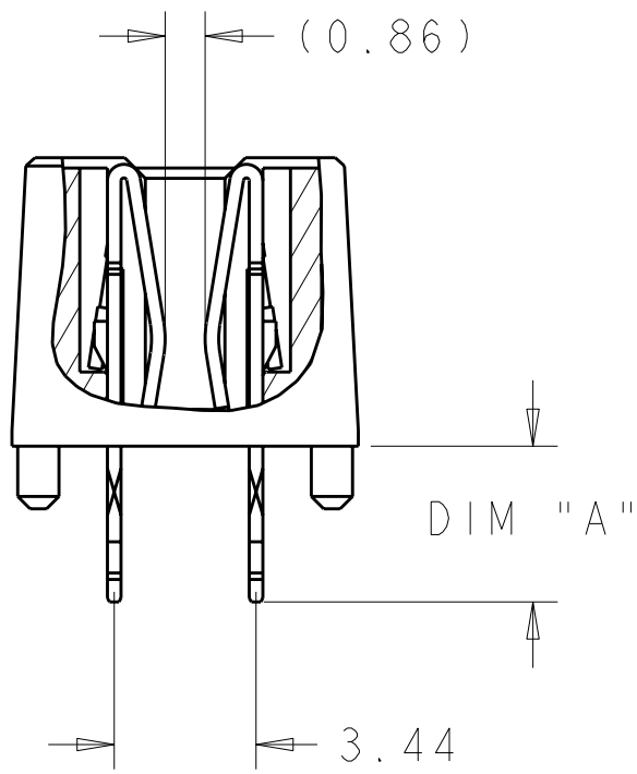
SECTION Z-Z
