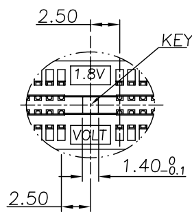
DETAIL A (1.8V) SCALE 2:1
