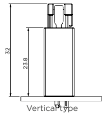
Vertical type
