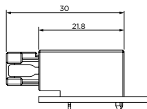
Horizontal type
