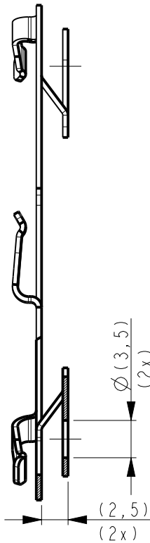
SECTION Q - Q
