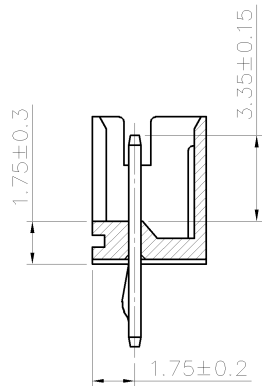
SECTION M-M
