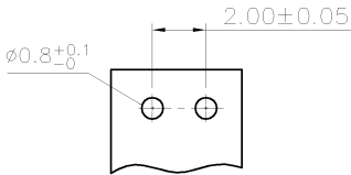
RECOMMENDED PCB LAYOUT (PCB THK=1.0MM~1.6MM)
