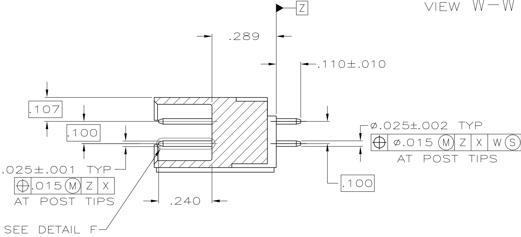
SECTION Z-Z
