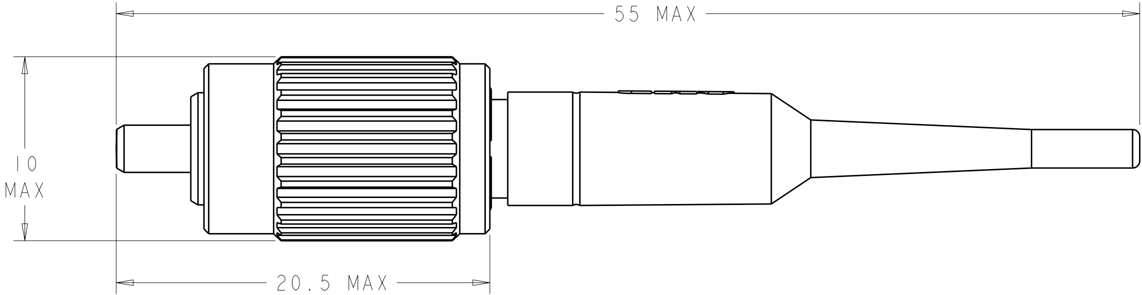
ASSEMBLED CONNECTOR
