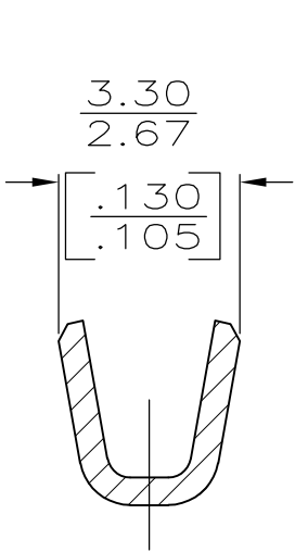
SECTION B-B SCALE 8:1
