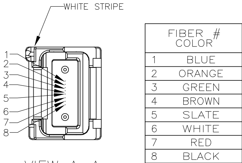
VIEW A-A LIGHTRAY MPX CONNECTOR FIBER PATH
