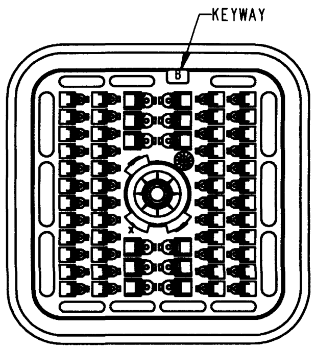
DRB16-60SBE-L018 KEY ARRANGEMENT -B-
