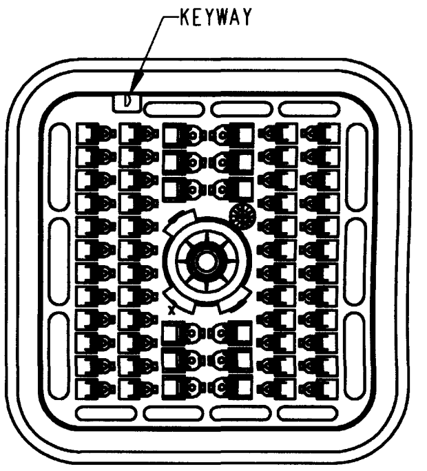
DRB16-60SDE-L018 KEY ARRANGEMENT -D-
