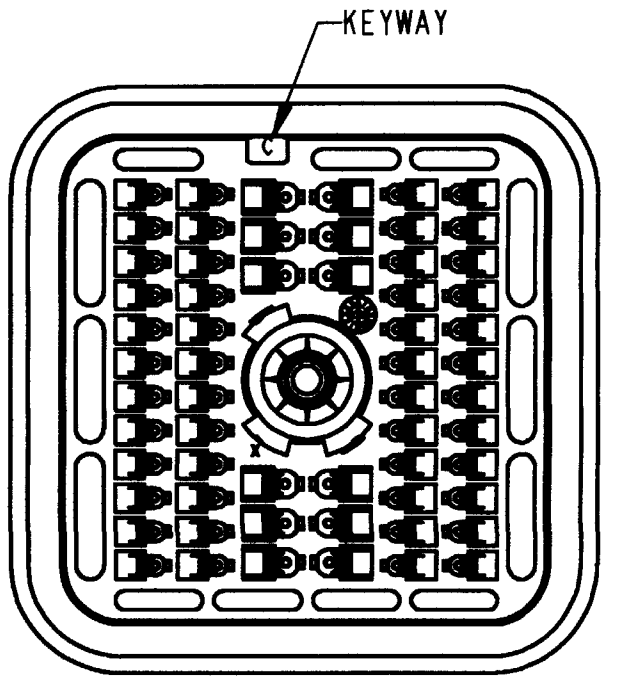
DRB16-60SCE-L018 KEY ARRANGEMENT -C-
