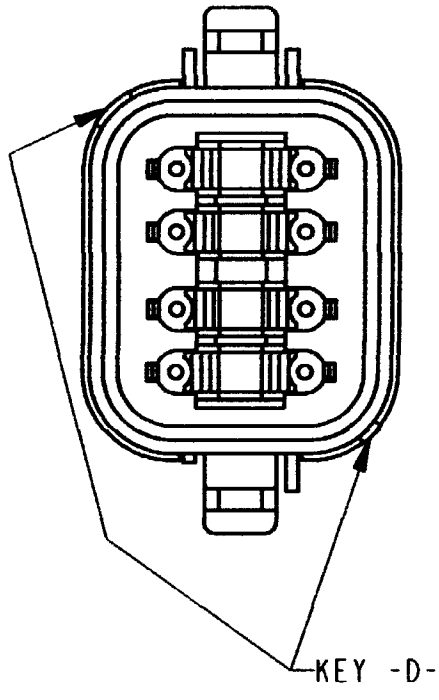
PART NO. DT06-08SD-CE01 KEY ARRANGMENT -D- COLOR: BROWN
