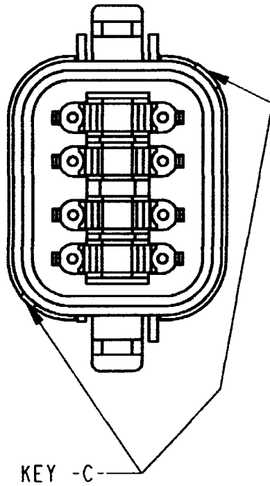
PART NO. DT06-08SC-CE01 KEY ARRANGMENT -C- COLOR: GREEN
