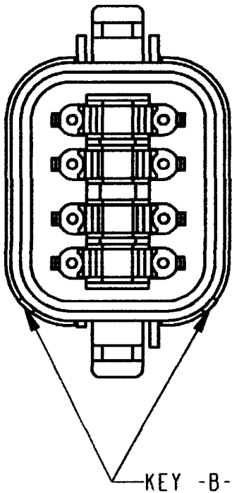
PART NO. DT06-08SB-CE01 KEY ARRANGMENT -B- COLOR: BLACK
